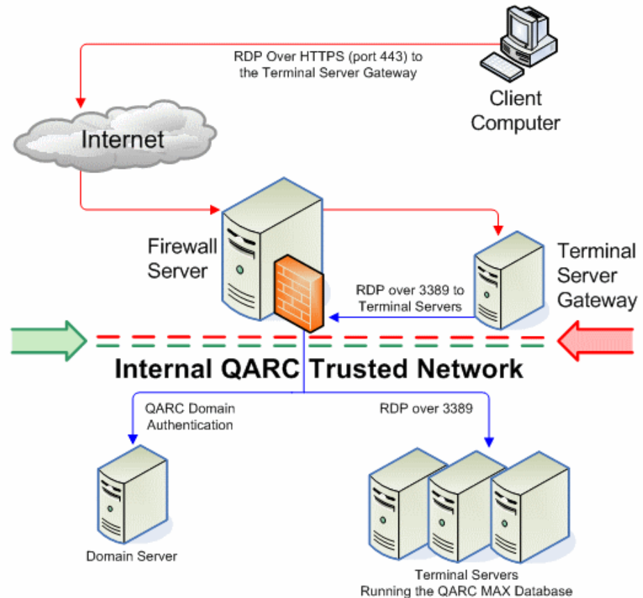
QARC Network Access Diagram – Remote Internet Desktop Users access QARC MAX Database using standard HTTPS to the Terminal Server Gateway (TSG). TSG communicates with Internal Terminal Servers via RDP 3389.
